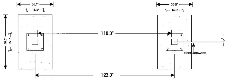
FOUNDATION PLAN Scale: 3/8" = 1'-0"
