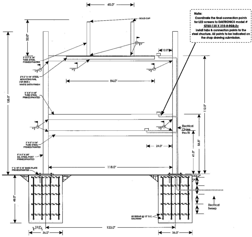
STRUCTURAL DETAIL Scale: 3/8" = 1'-0"
